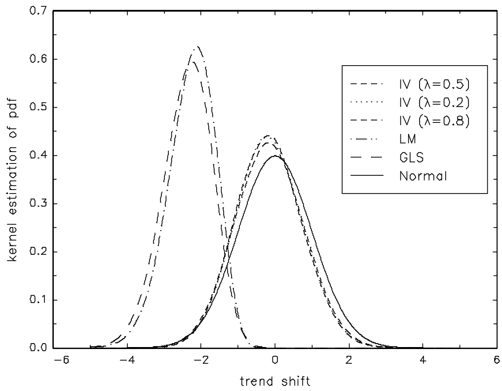
Figure 2. Estimated pdf ( T = 500 )
