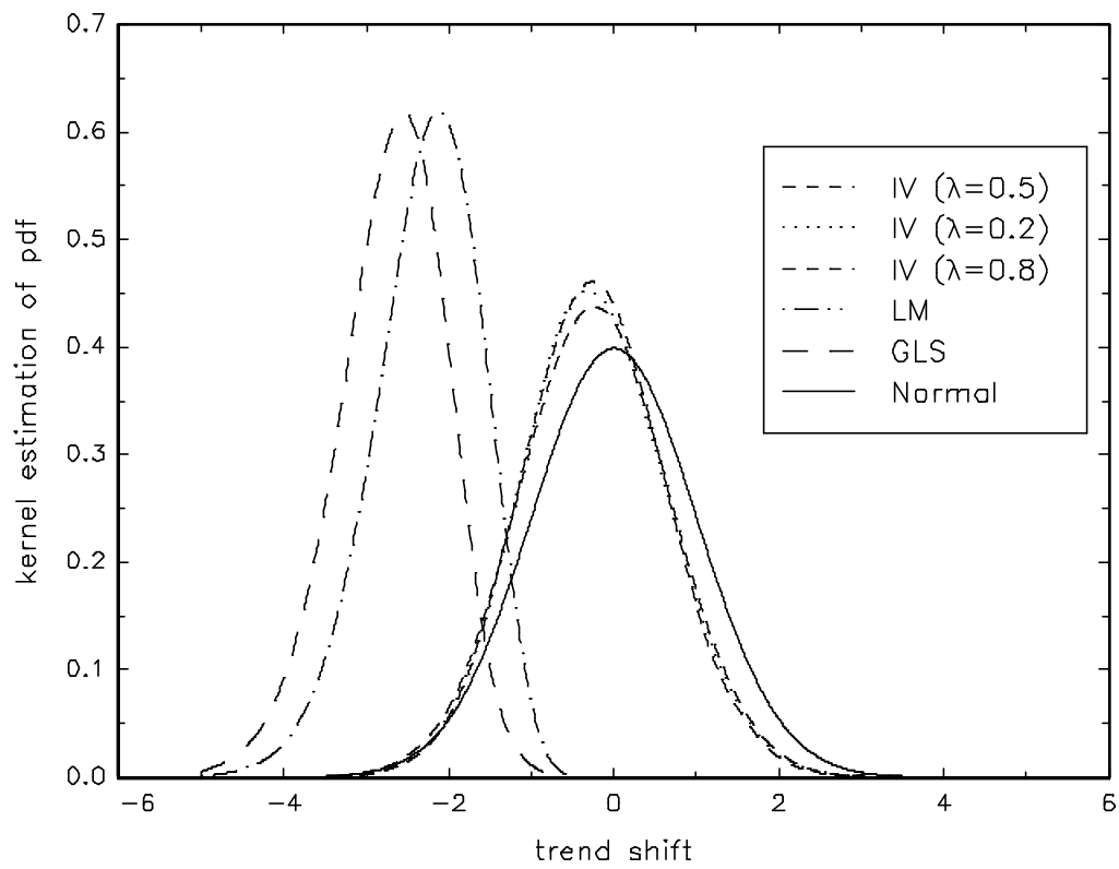
Figure 1. Estimated pdf ( T = 100 )
